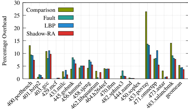
Fig. 9: Epilogue Micro-Optimizations
